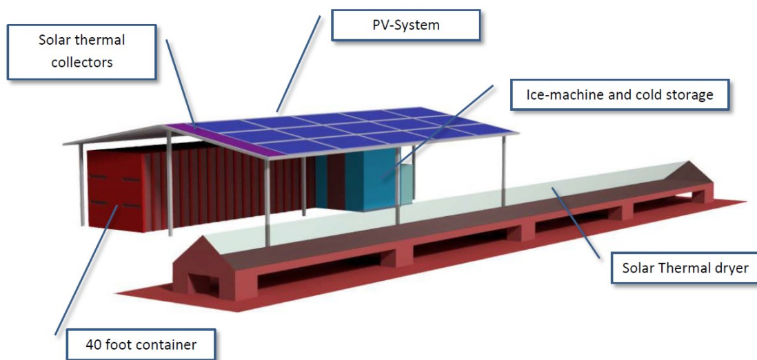
Fig. 3: Simplified system concept with photovoltaic system, solar collectors, 40-foot container, ice machine and small cold room for the flake ice, and solar thermal dryer.
